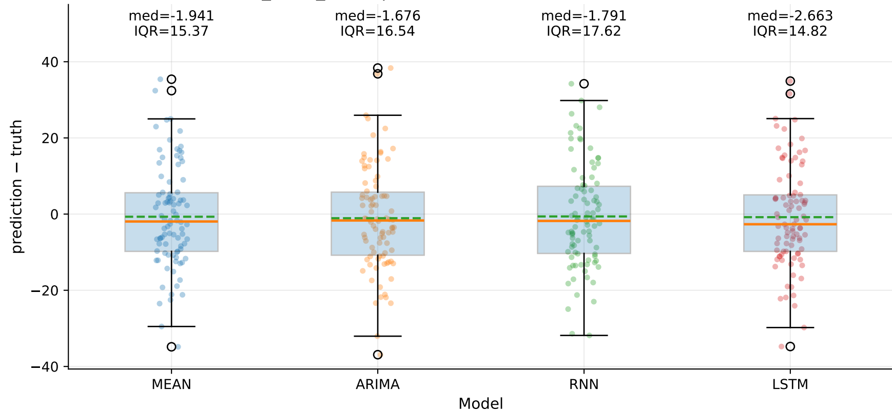
M9_YLUR_SHUR | Signed error by model — Yd (step=1)
