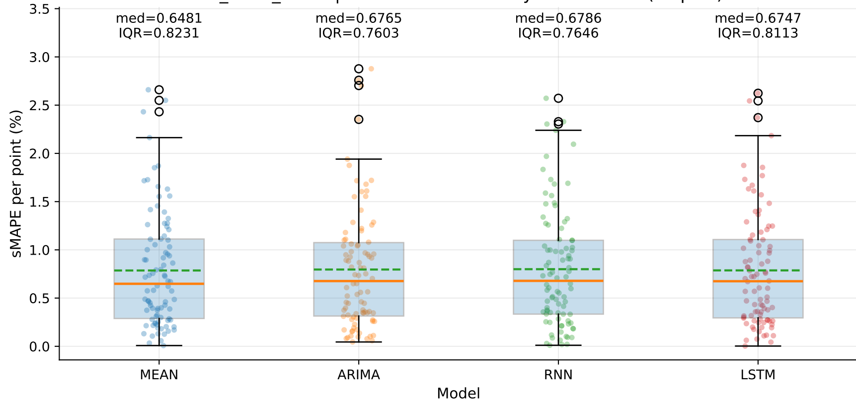
M9_YLUR_SHUR | sMAPE distribution by model — Yd (step=1)
