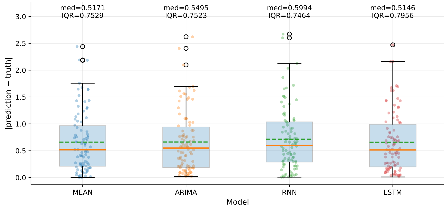
M9_YLUR_SLUR | Absolute error by model — TSEC (step=1)
