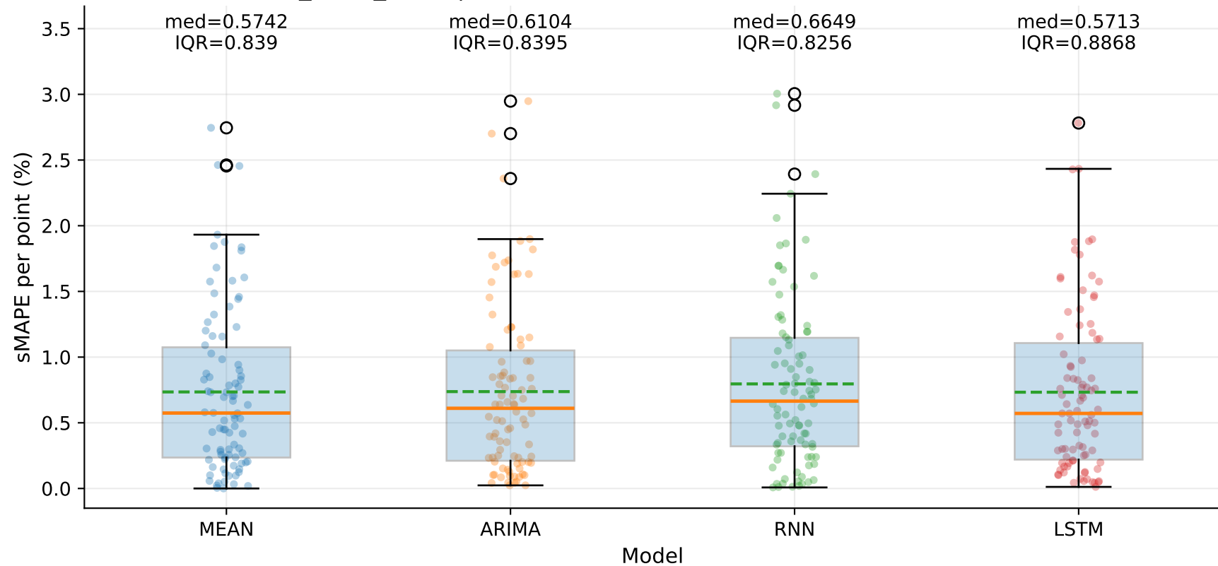
M9_YLUR_SLUR | sMAPE distribution by model — TSEC (step=1)
