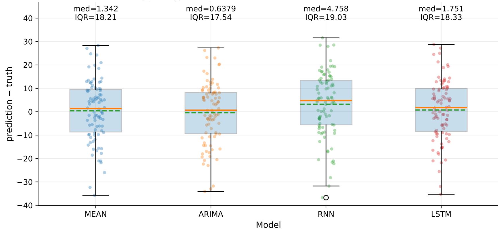
M9_YLUR_SLUR | Signed error by model — TSE (step=1)
