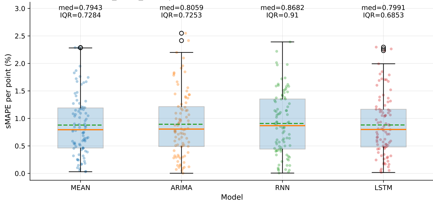
M9_YLUR_SLUR | sMAPE distribution by model — Yd (step=1)
