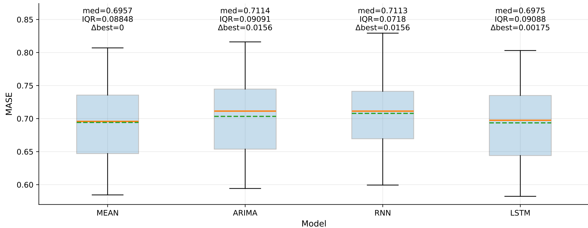
MASE across cases by model — TSE (step_1)
