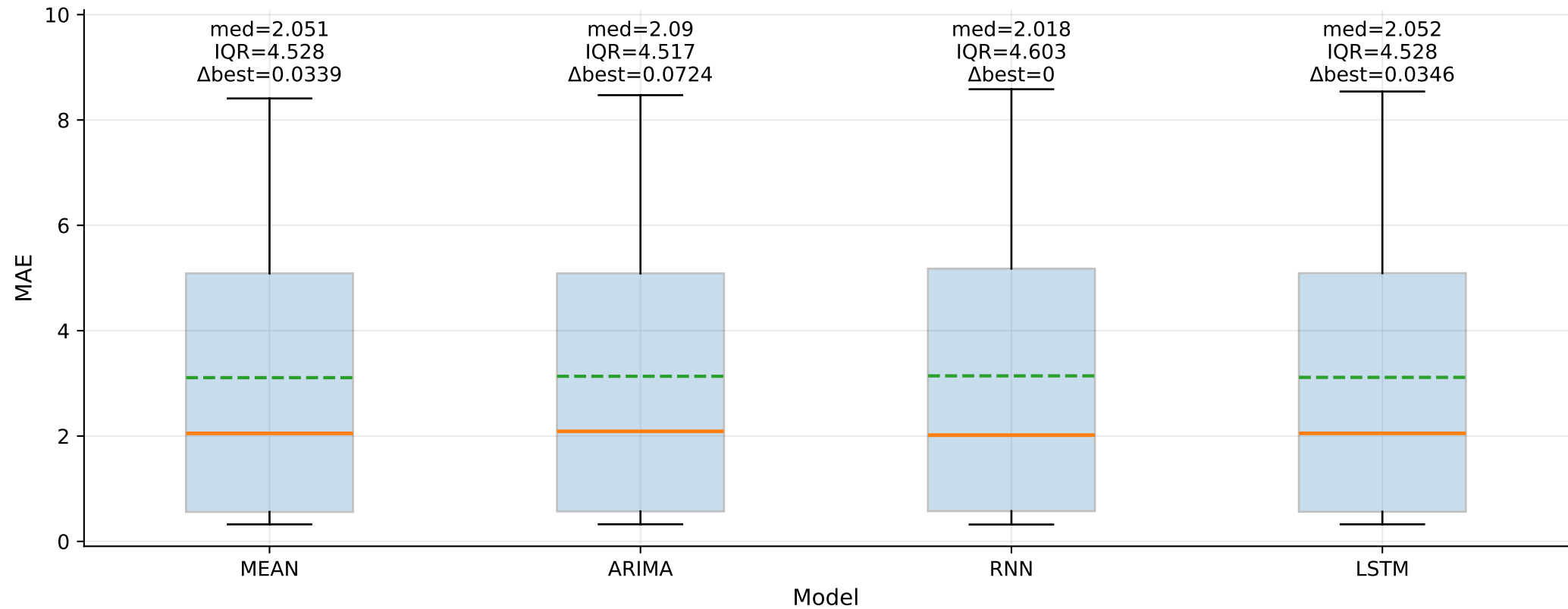
MAE across cases by model — TSEC (step_1)
