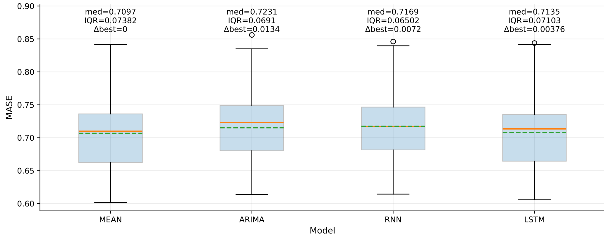
MASE across cases by model — TSEC (step_1)
