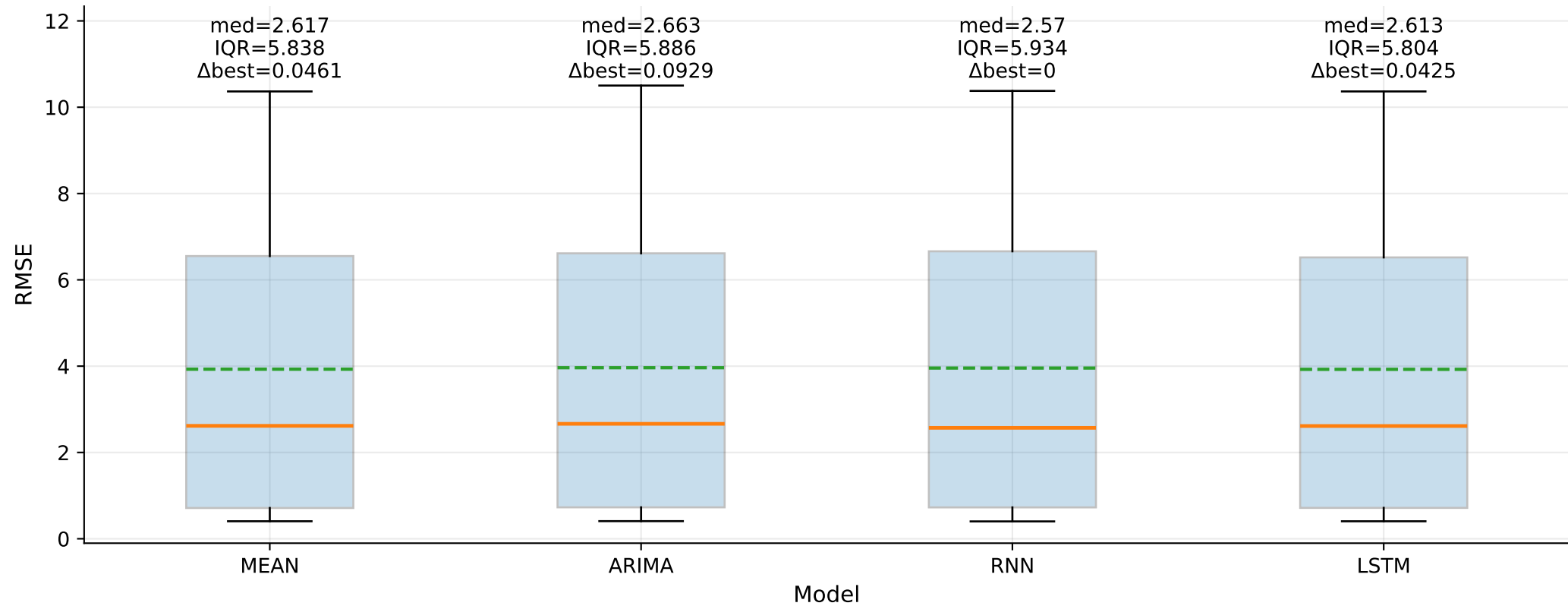
RMSE across cases by model — TSEC (step_1)
