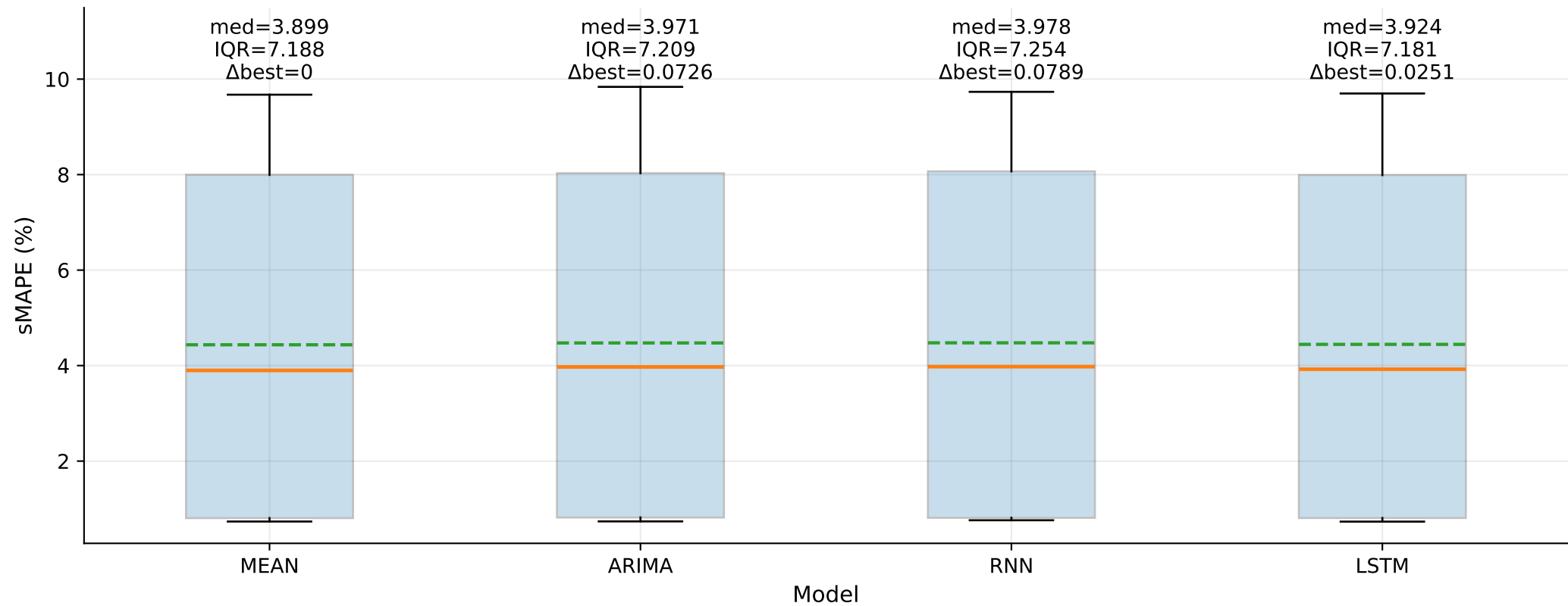
sMAPE (%) across cases by model — TSEC (step_1)
