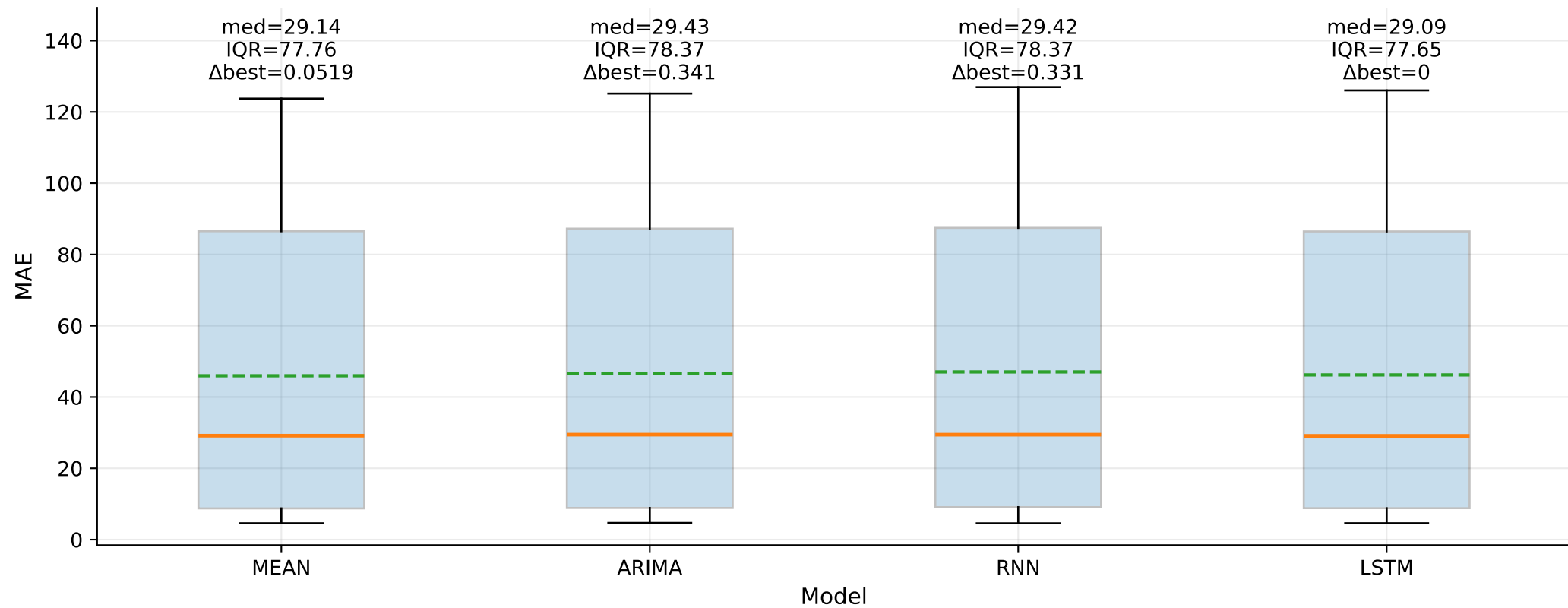
MAE across cases by model — Yd (step_1)
