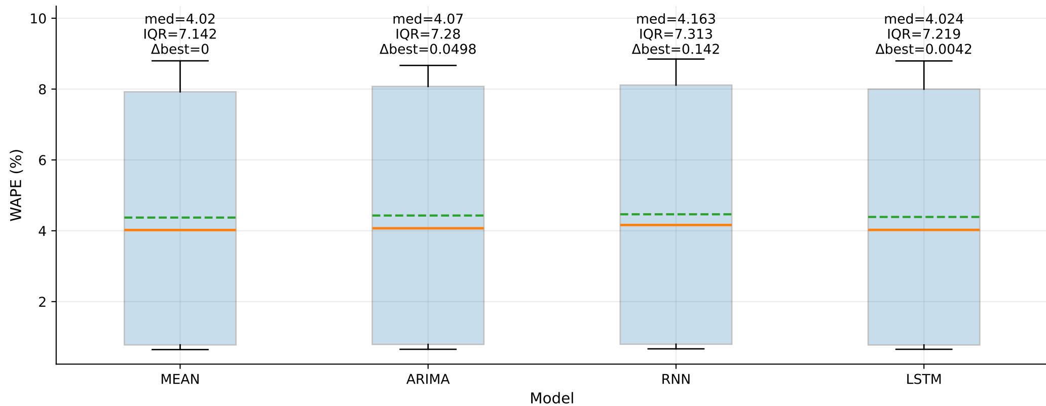
WAPE (%) across cases by model — Yd (step_1)
