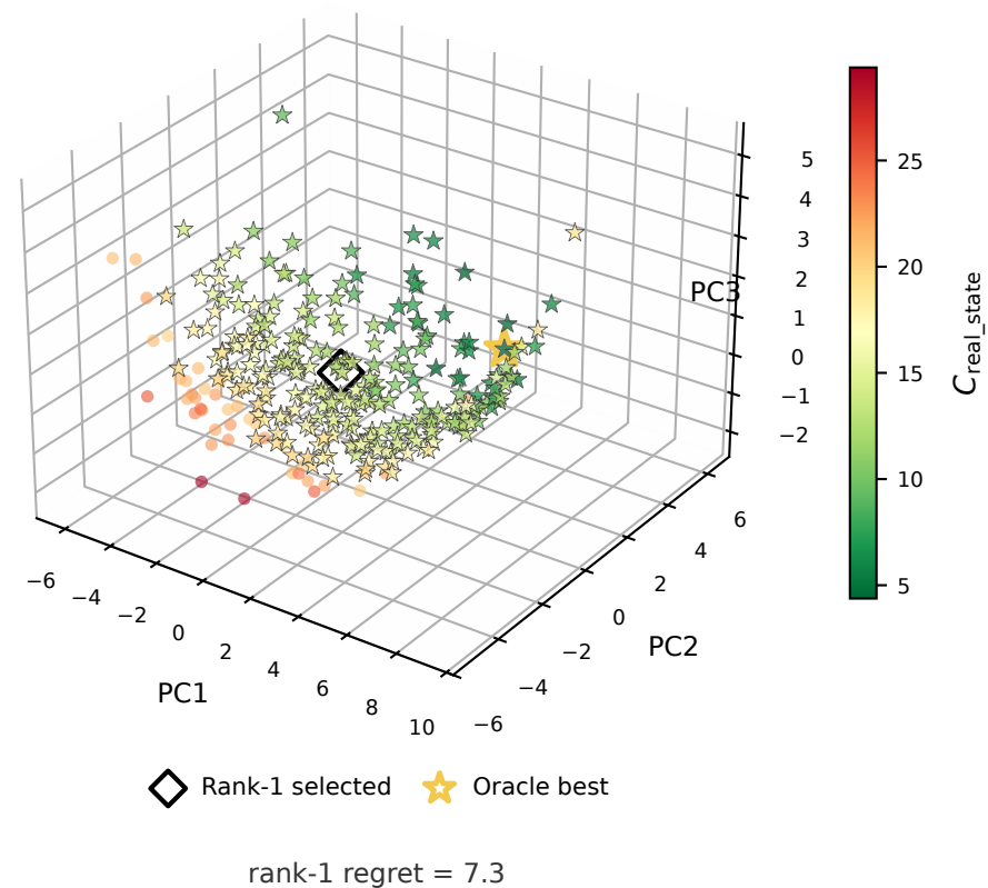
(b) CEM pool in latent space (pair 51)
