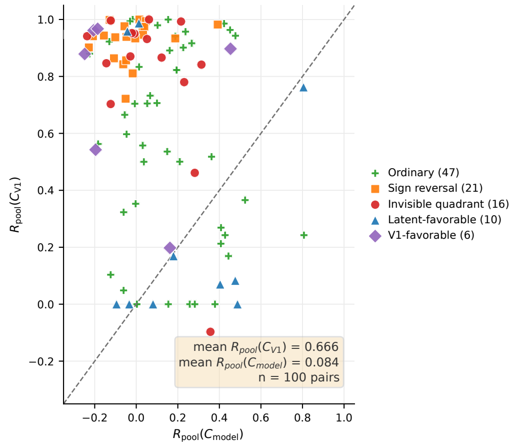
(a) V1 attribution across PushT pairs
