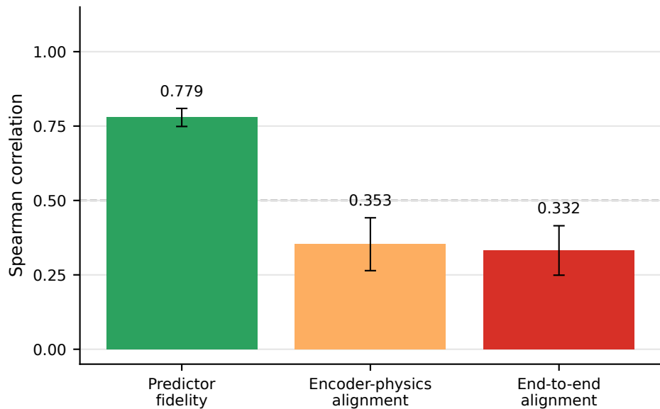
(b) Per-pair three-cost attribution (offset 50, \pm SEM)
