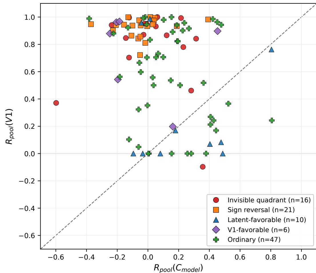
V1 Attribution of CEM-Pool Ranking
