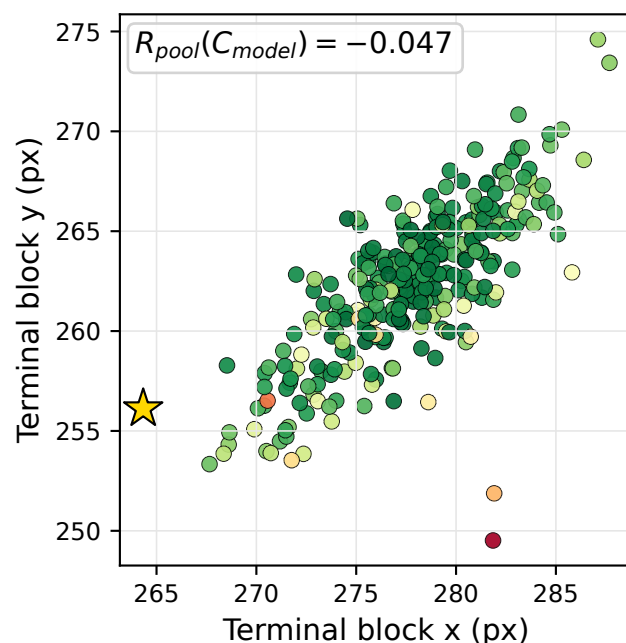
(b) CEM Pool (learned cost)
