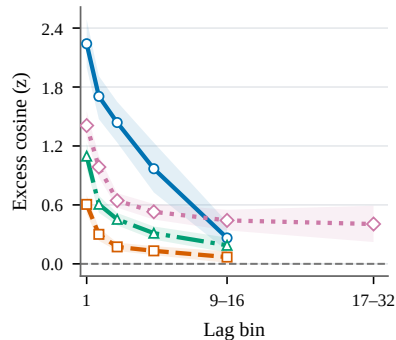
(a) Semantic
