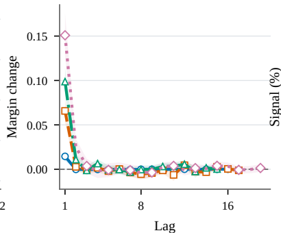
(b) Influence
