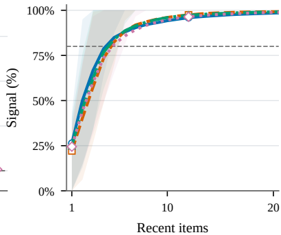
(c) Coverage
