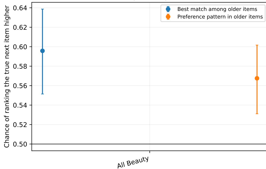
Can older history identify the next item?
