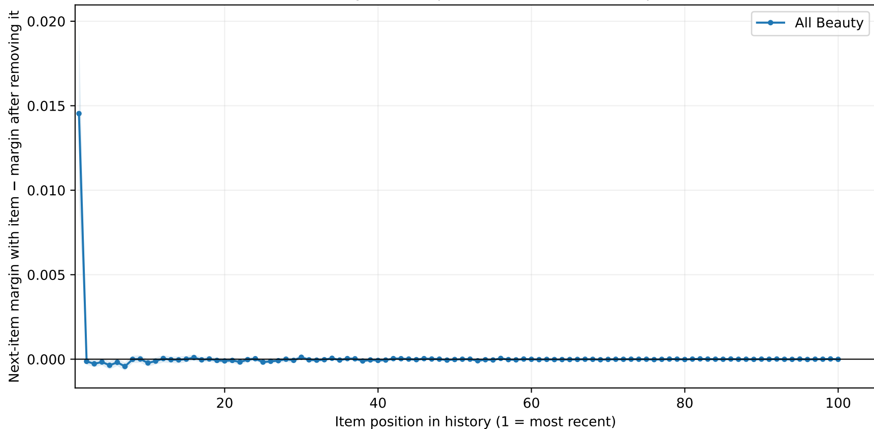
How each history item helps or hurts the next-item prediction
