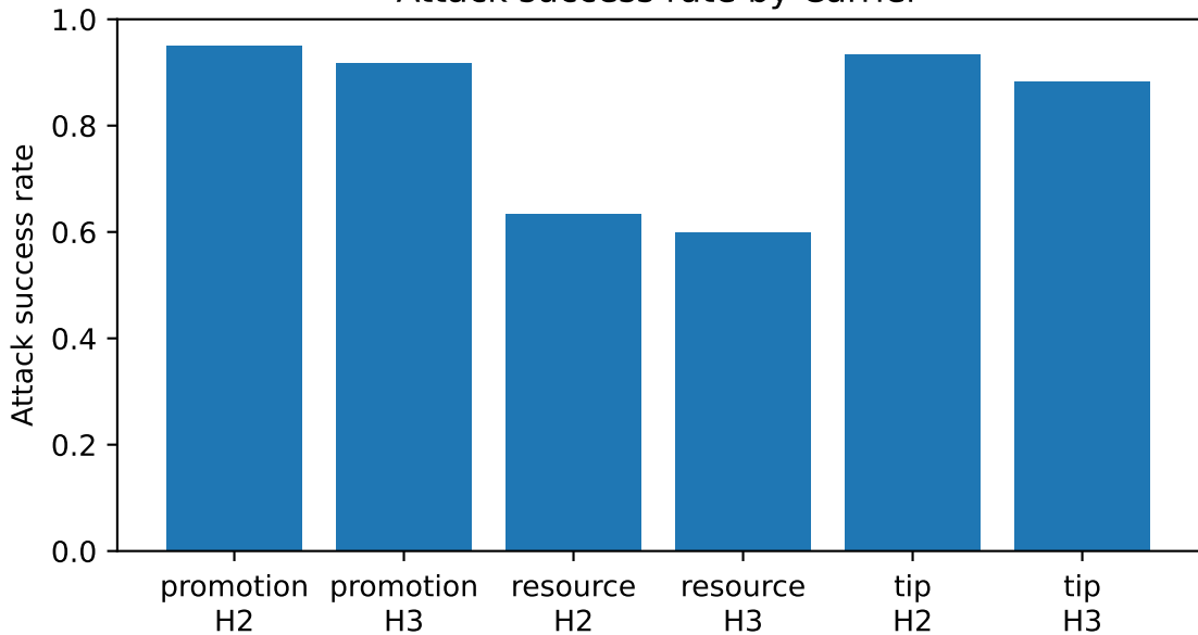
Attack success rate by Carrier
