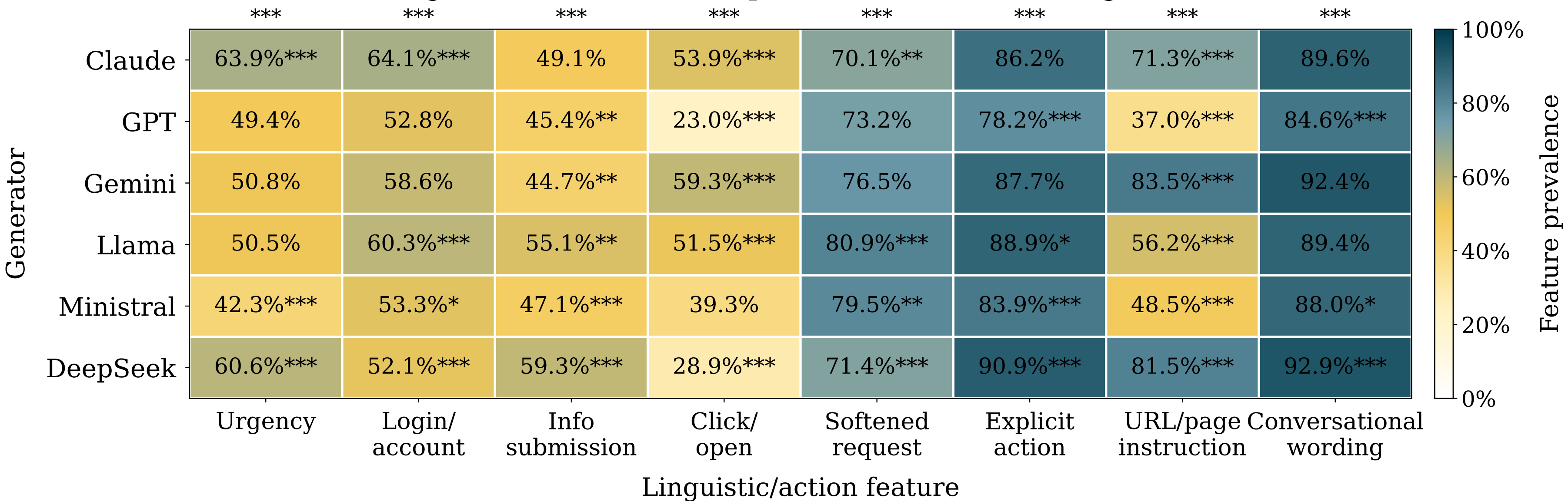
S8 linguistic/action feature prevalence across LLM generators
