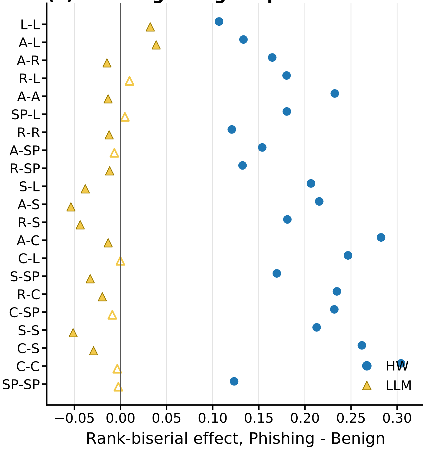
(a) Phishing-benign separation
