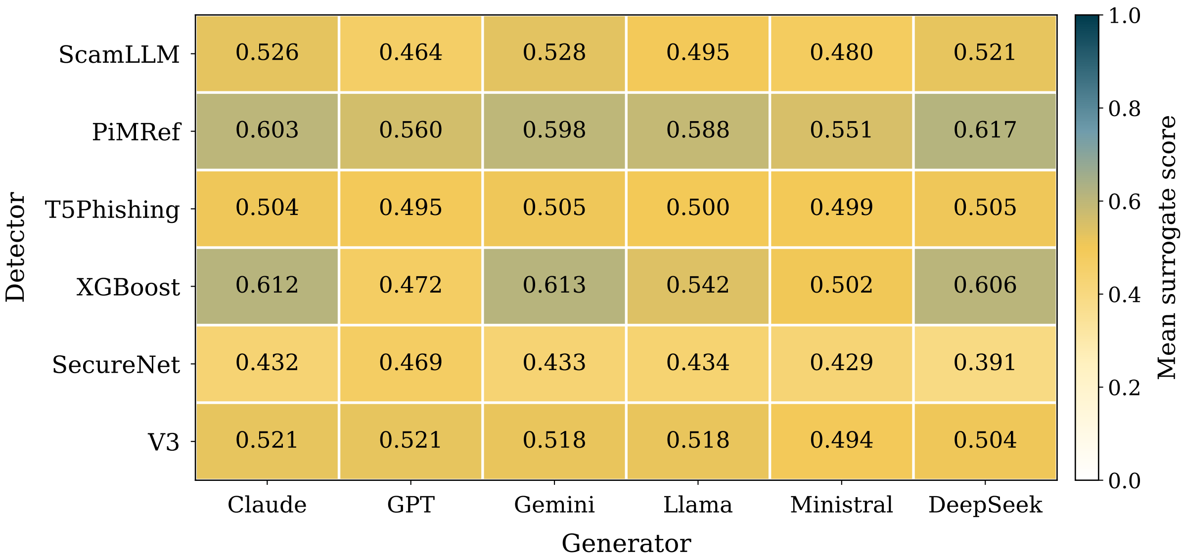
Detector-specific continuous surrogate score by S8 generator
