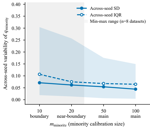
Logistic Regression
