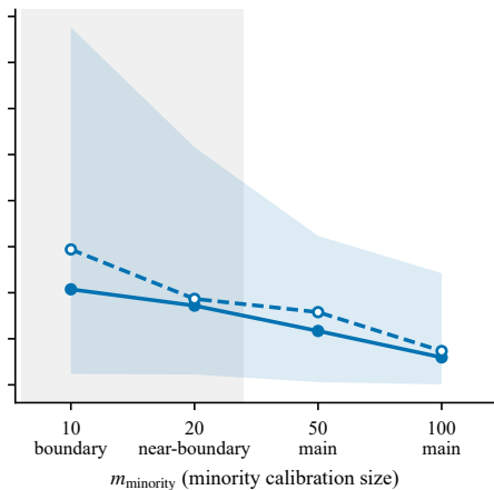
XGBoost
