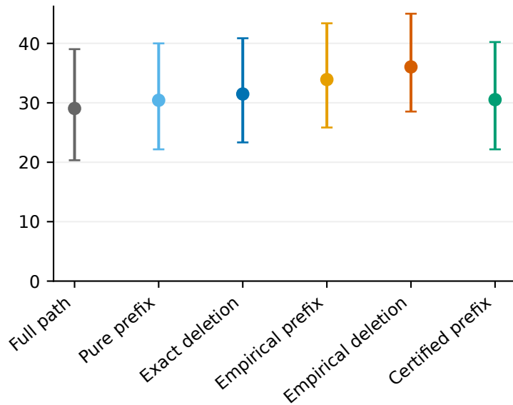
Reference coverage (%)
