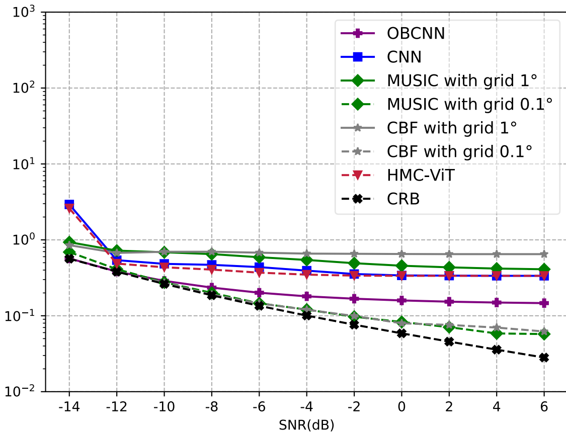
RMSE of DOA estimates(degree)
