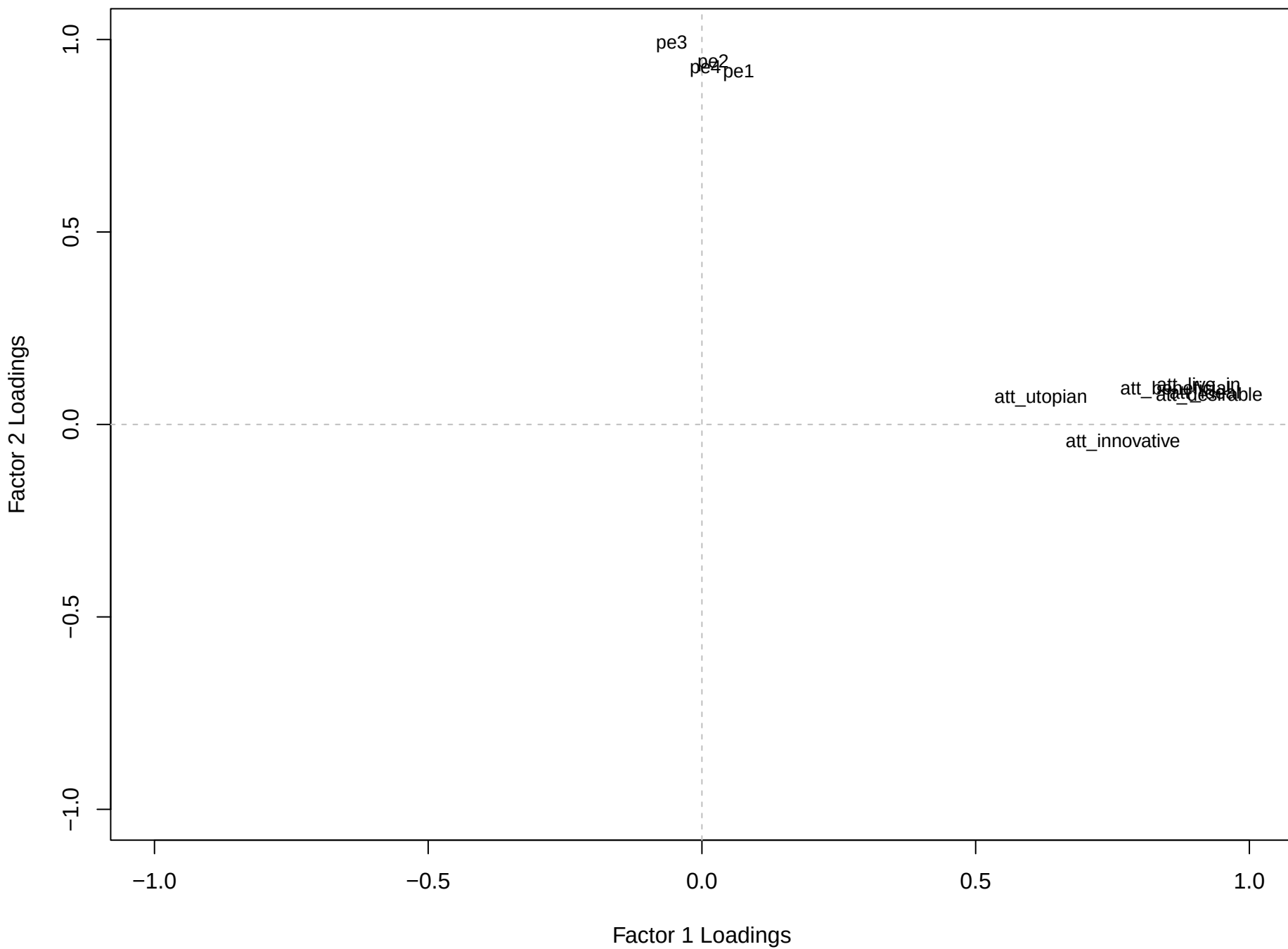
Factor Loadings Plot (2-Factor Solution)
