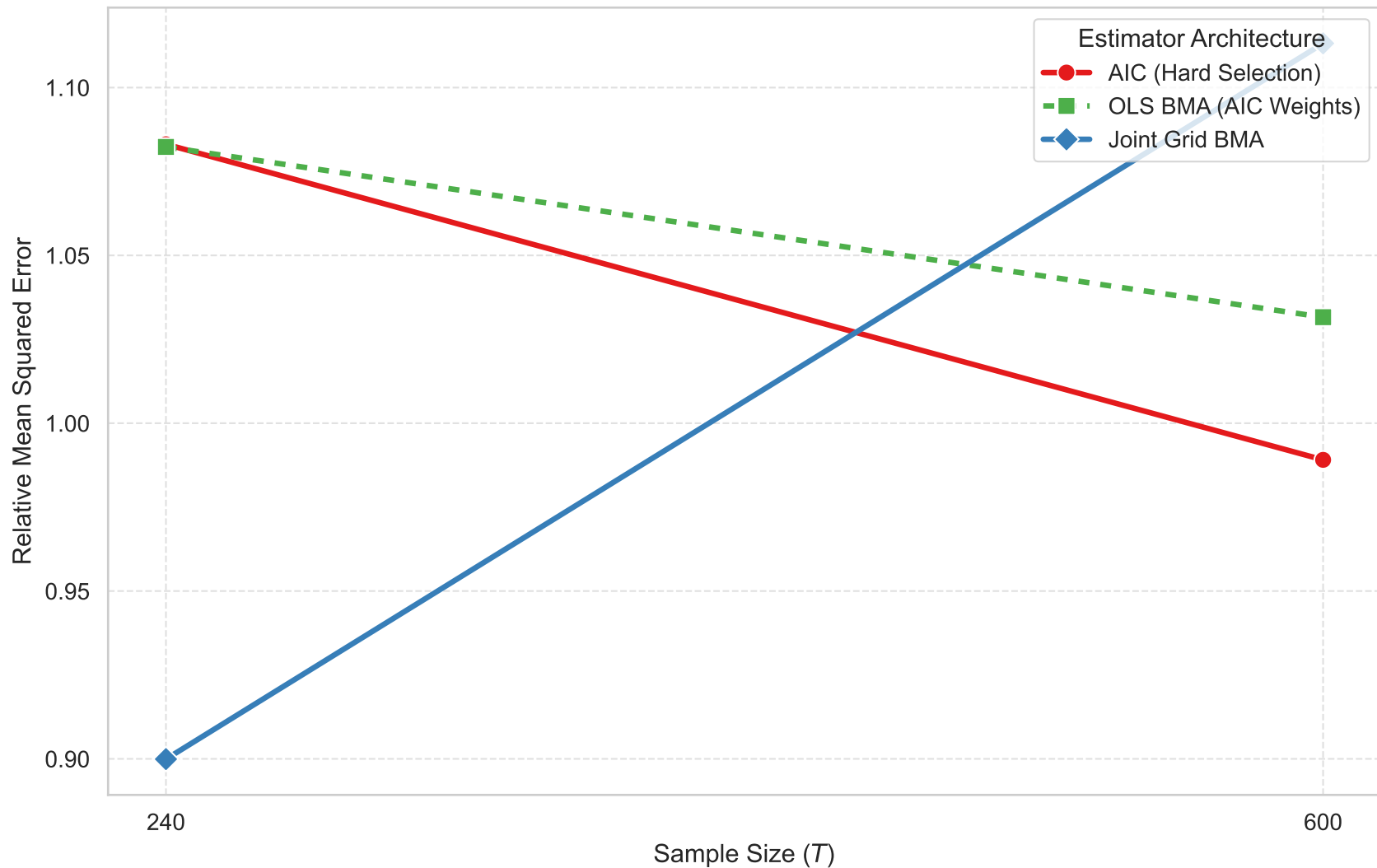
Asymptotic Convergence: BMA vs. ~Hard Selection ( p_0 = 4 )
