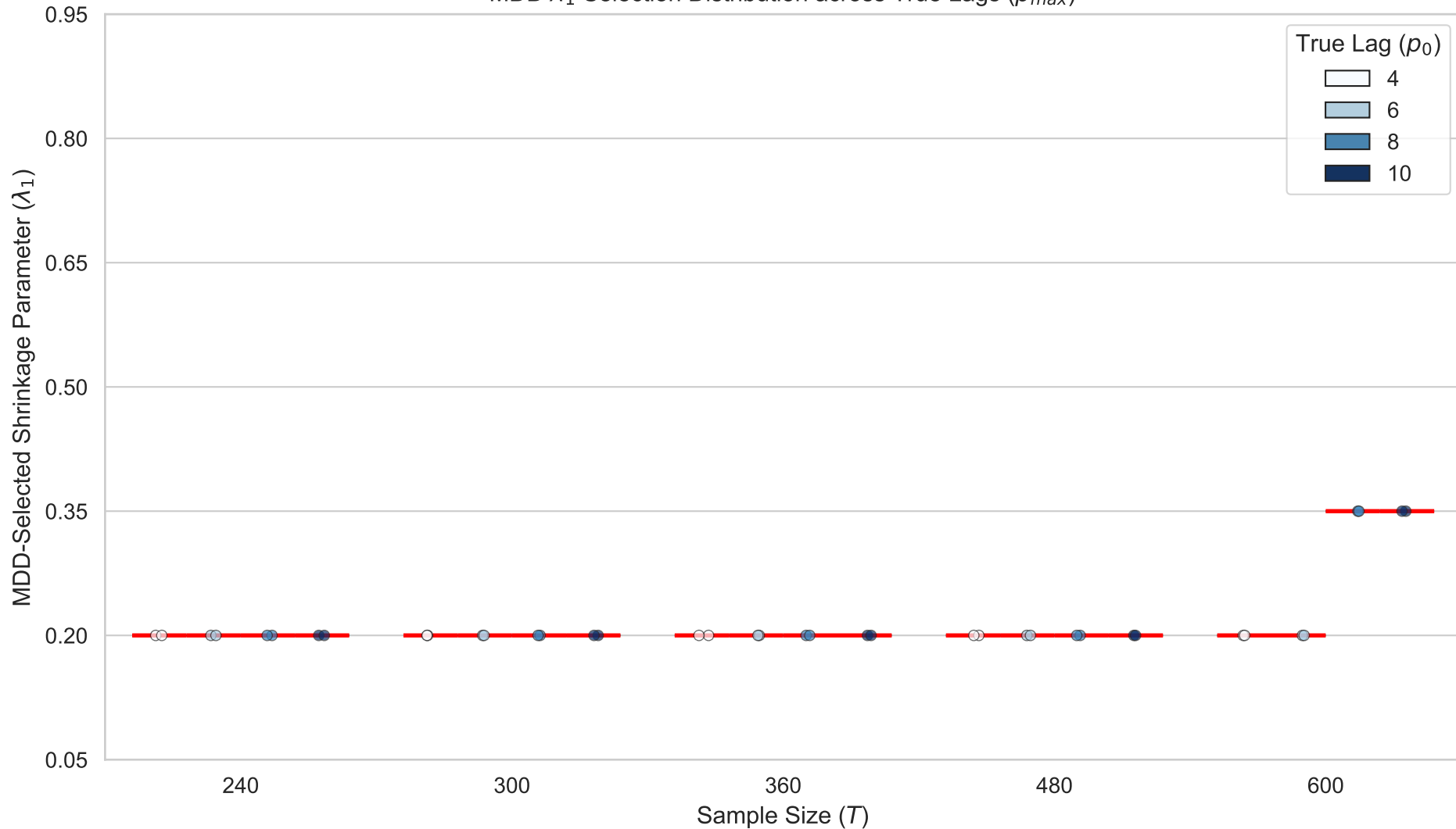
MDD \lambda_1 Selection Distribution across True Lags ( p_{max} )
