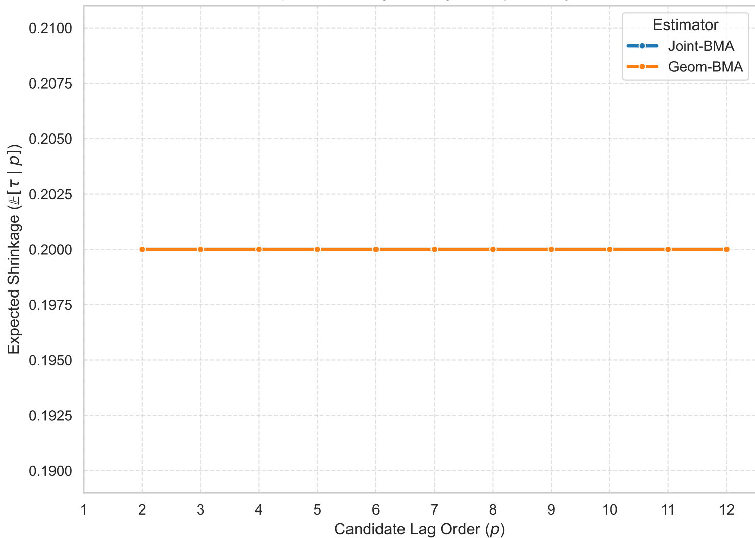
Optimal Shrinkage vs. Lag Order ( T = 240 )
