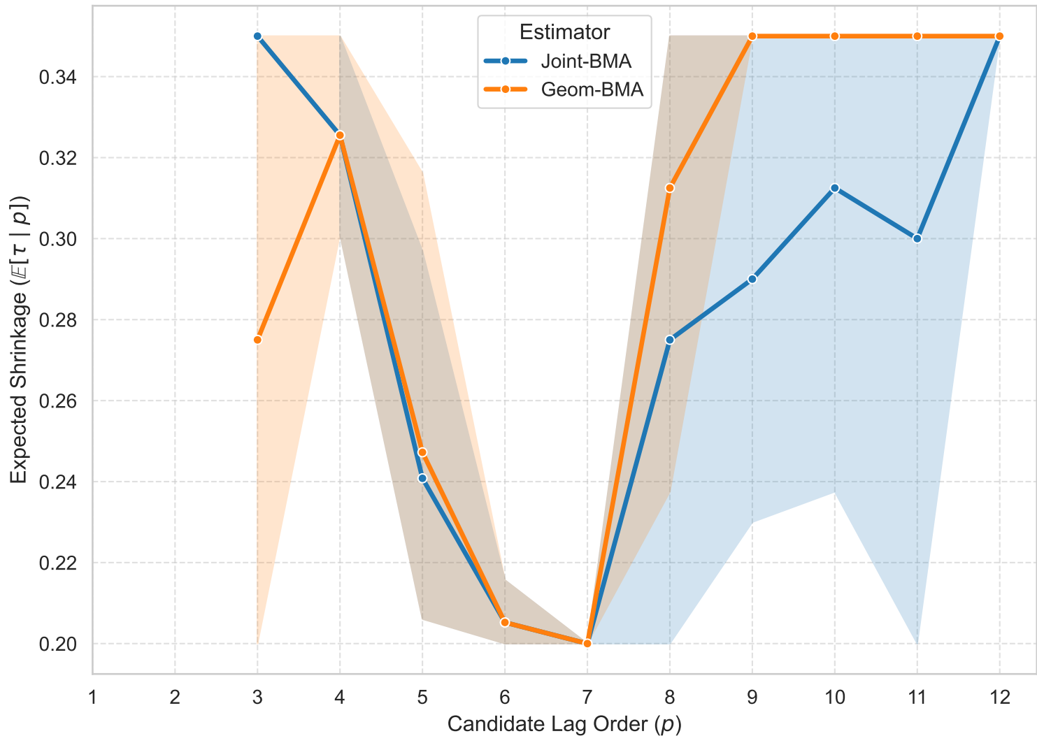
Optimal Shrinkage vs. Lag Order ( T = 600 )
