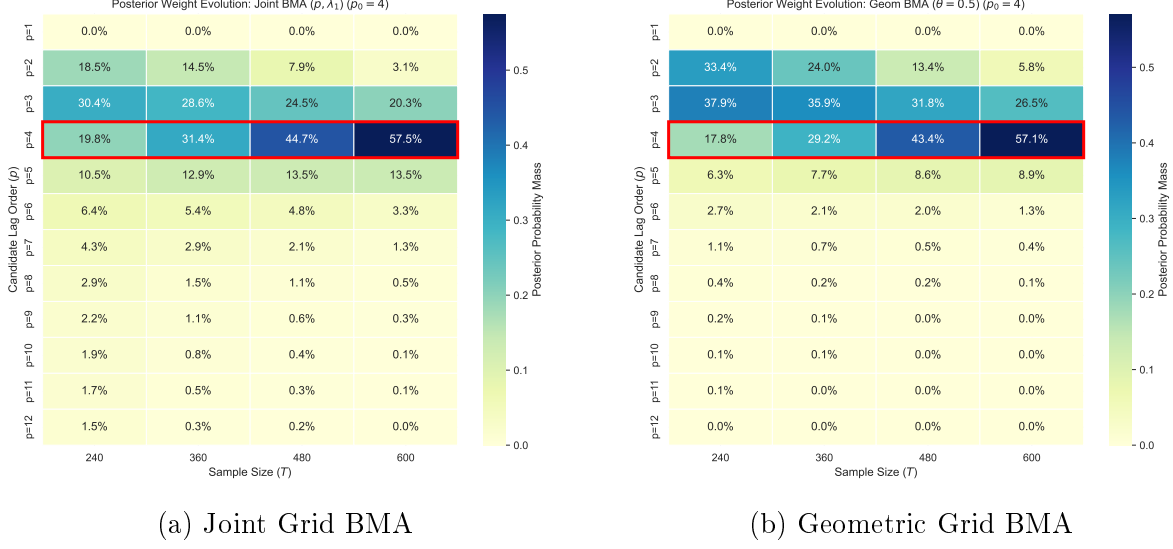
Figure 2: Posterior Weight Evolution for the two BVAR-based BMAs ( p_0 = 4 ).
