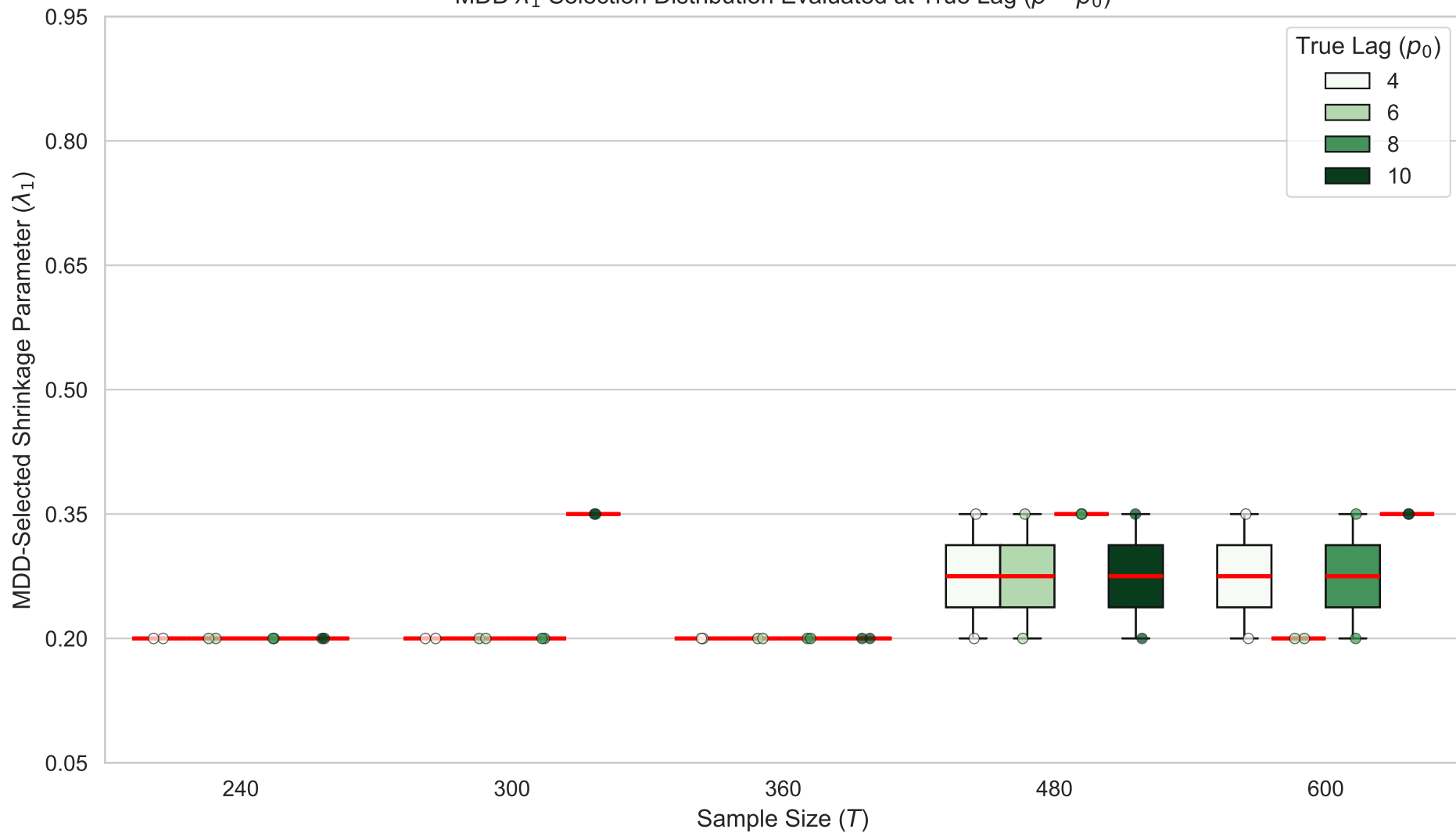
MDD \lambda_1 Selection Distribution Evaluated at True Lag ( p = p_0 )
