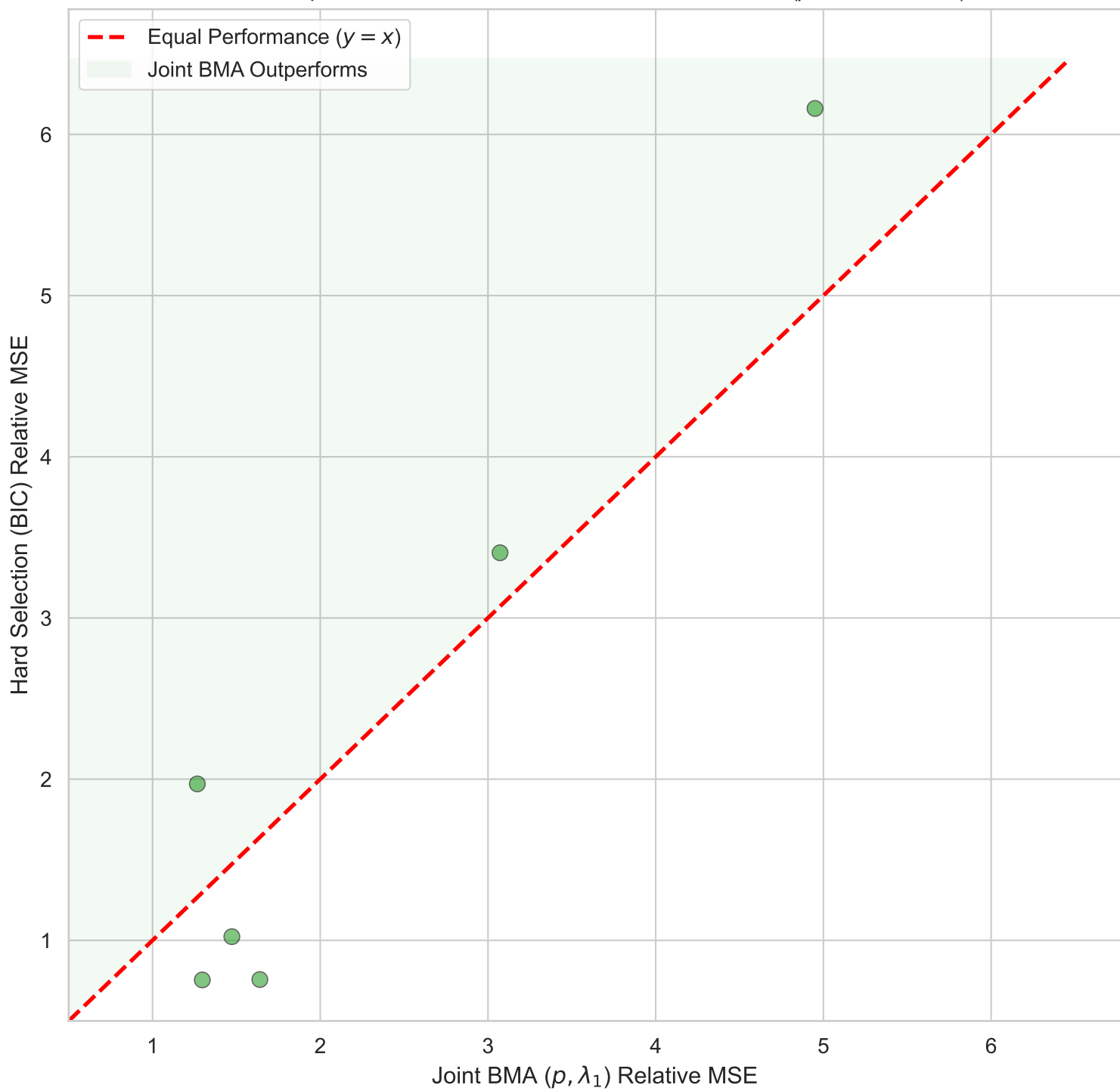
Catastrophe Avoidance: Joint BMA vs. ~Hard Selection ( p_0 = 4 , T = 96 )
