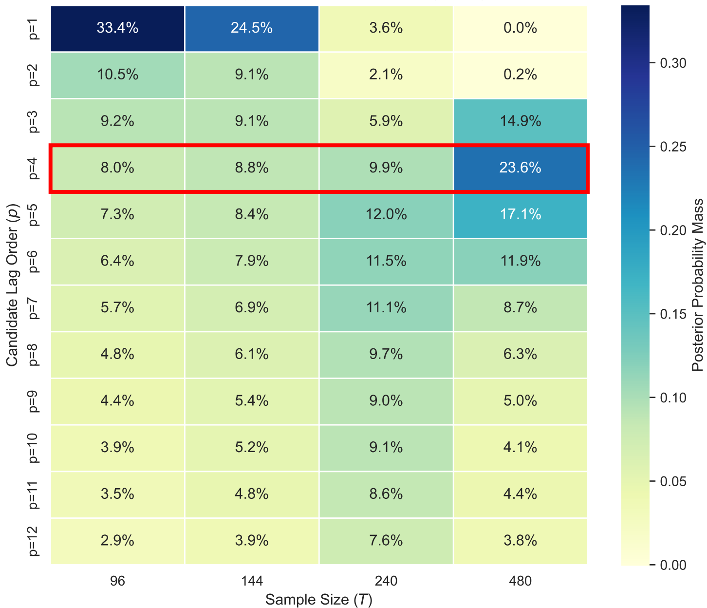
Posterior Weight Evolution of SOTA-BMA ( p_0 = 4 )
