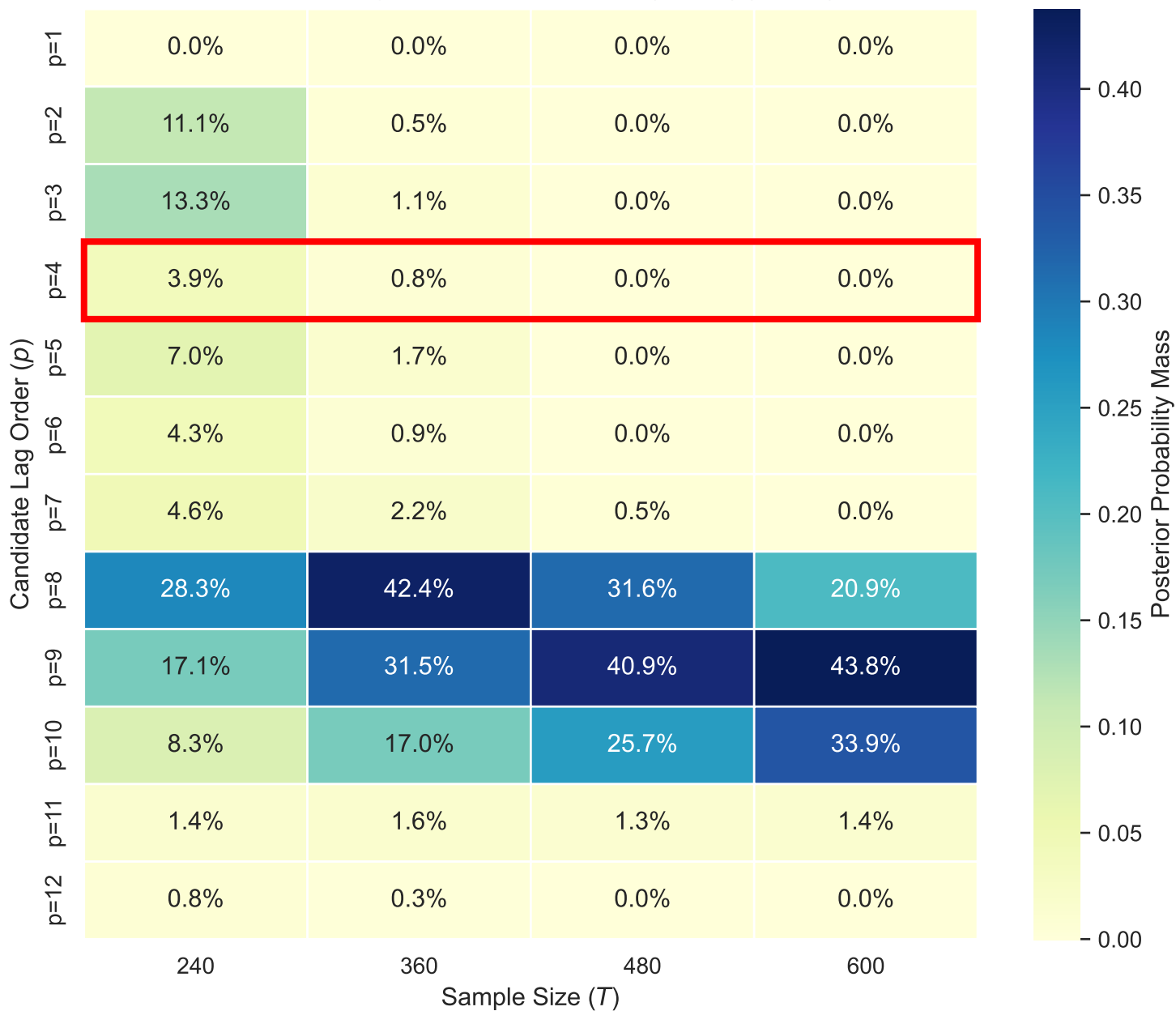
Posterior Weight Evolution: OLS BMA (AIC-W) ( p_0 = 4 )
