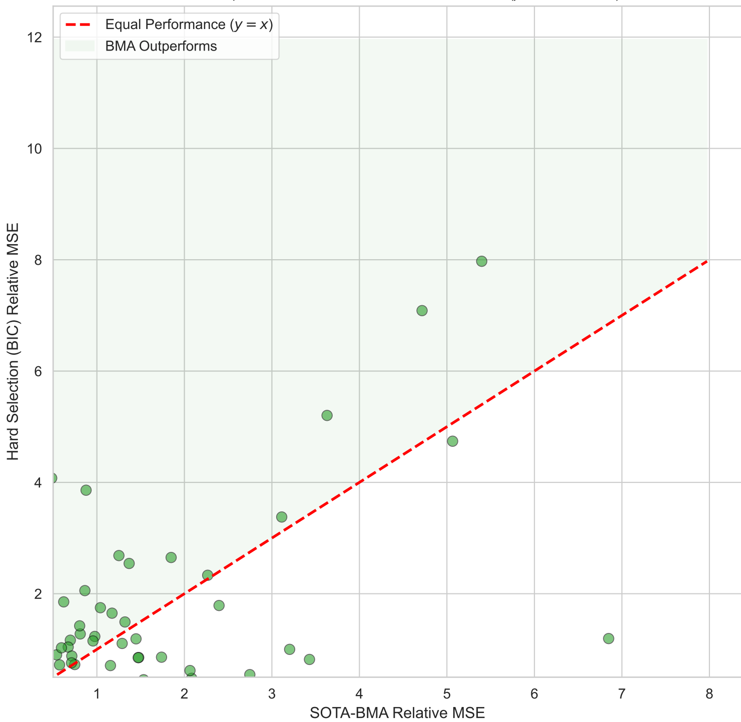
Catastrophe Avoidance: BMA vs. Hard Selection ( p_0 = 4, T = 96 )
