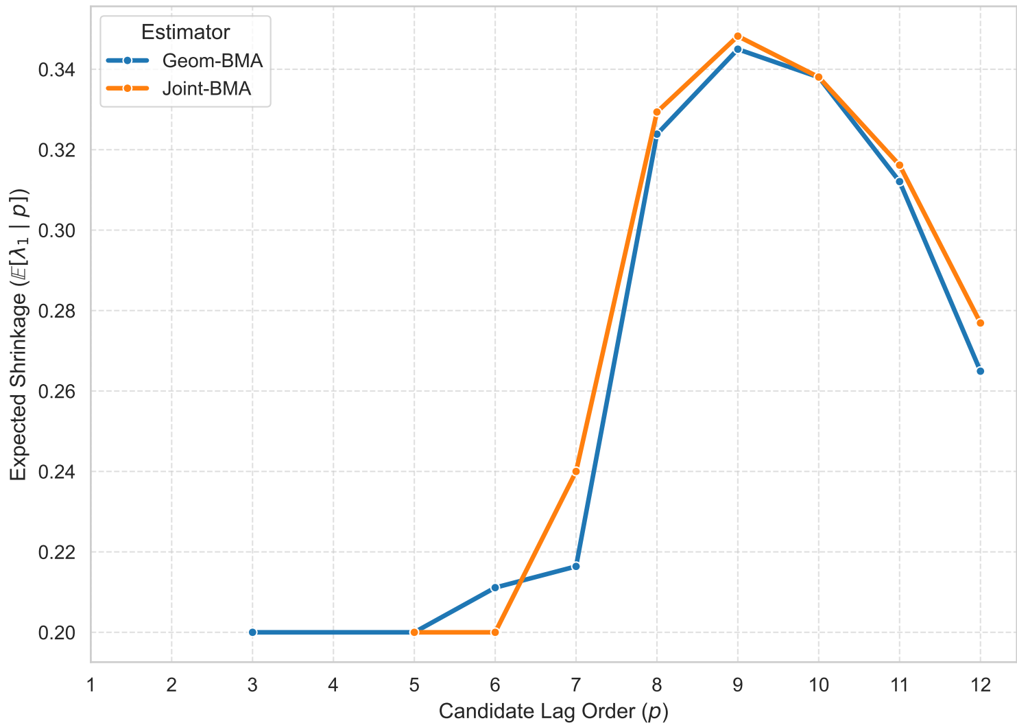
Optimal Shrinkage vs. Lag Order ( T = 600, p_0 = 10 )
