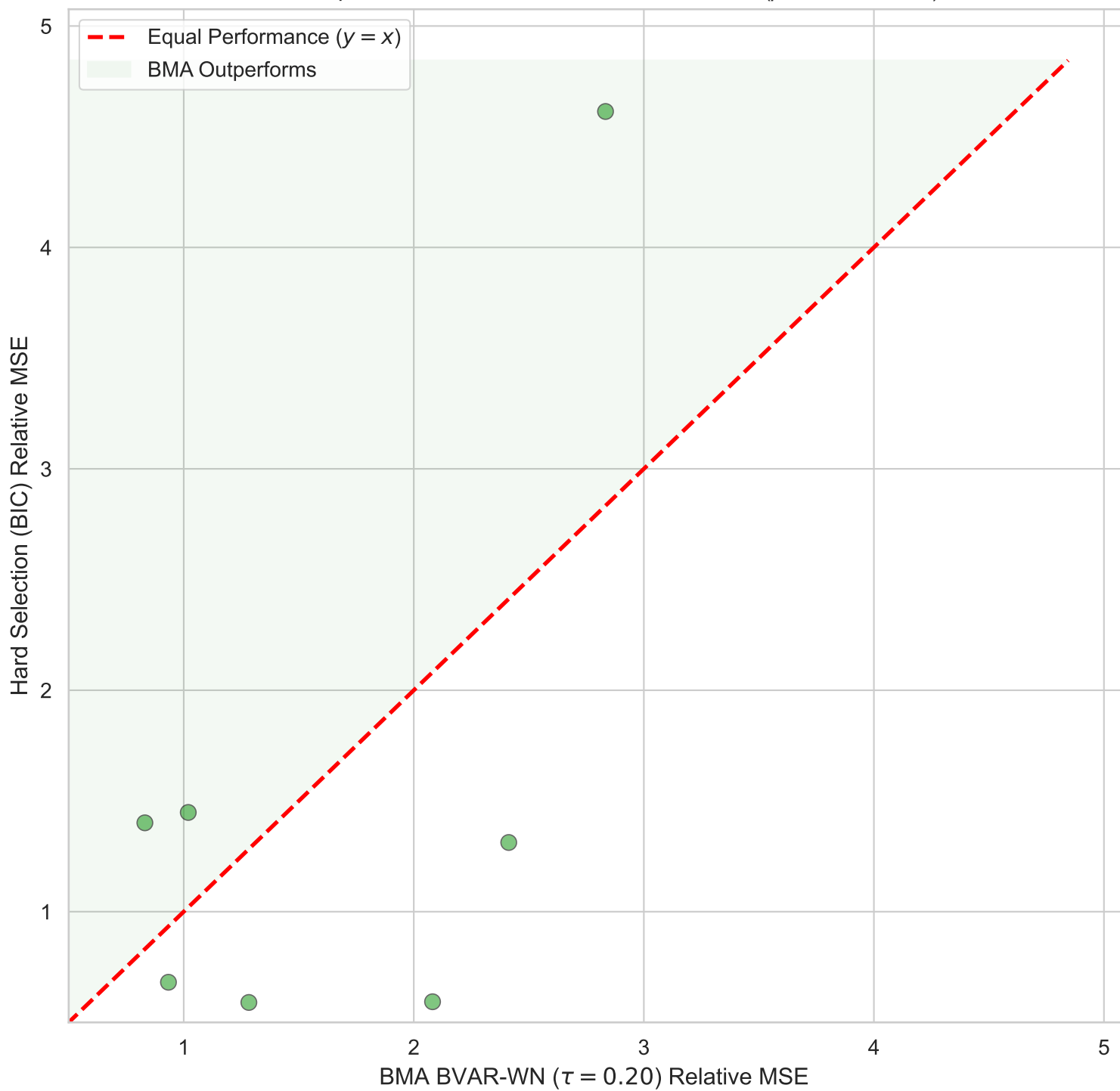
Catastrophe Avoidance: BMA vs.~Hard Selection ( p_0 = 4, T = 96 )
