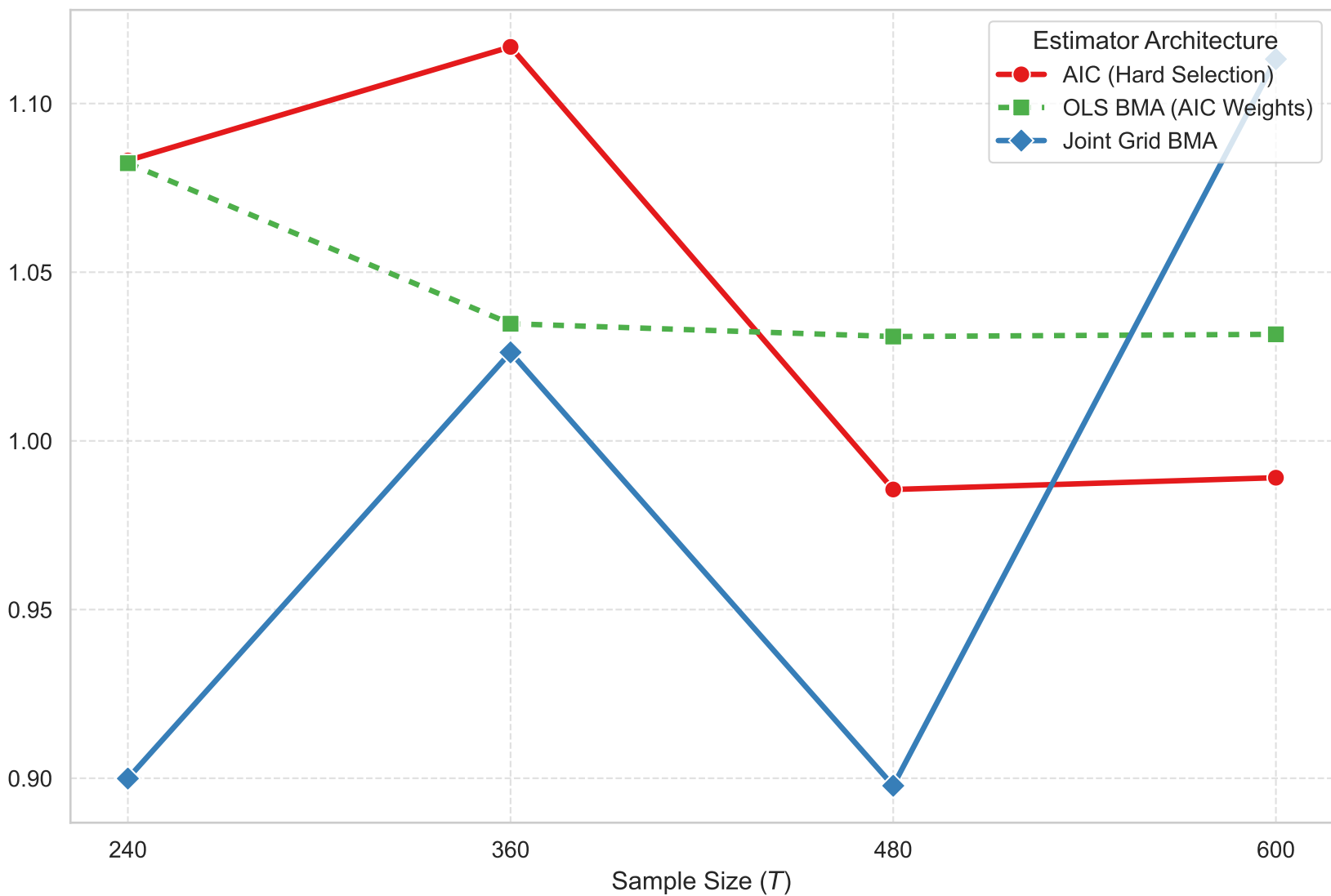
Relative Mean Squared Error
