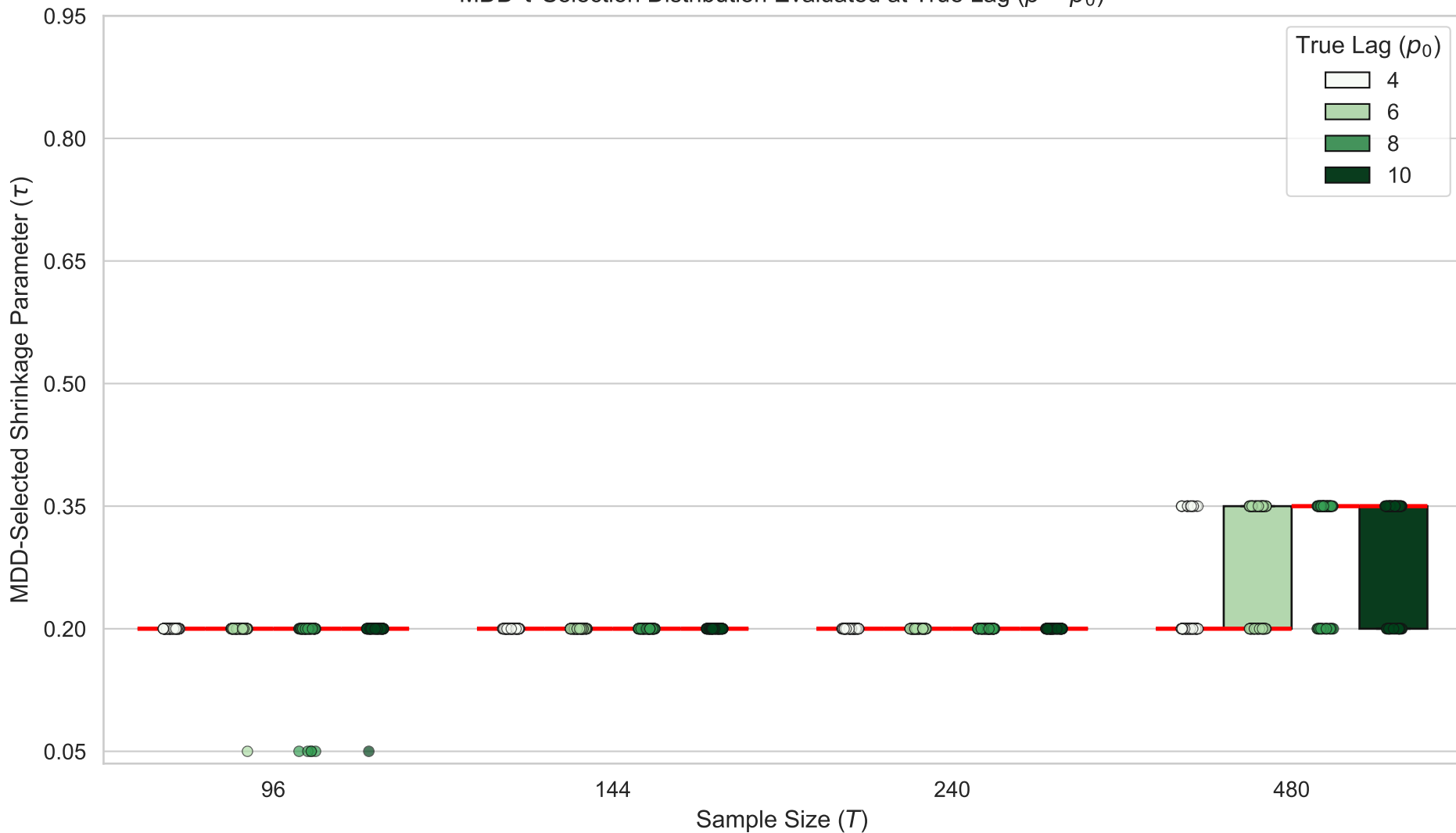
MDD \tau Selection Distribution Evaluated at True Lag ( p = p_0 )
