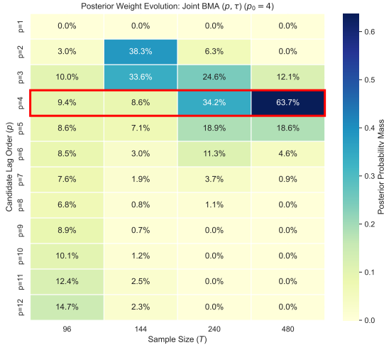
(c) Joint BMA ( p, \tau )
