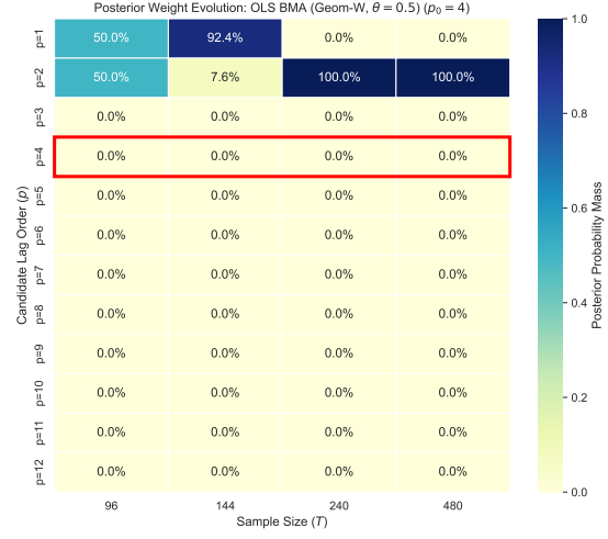
(b) OLS BMA (Geom-W, \theta = 0.5 )
