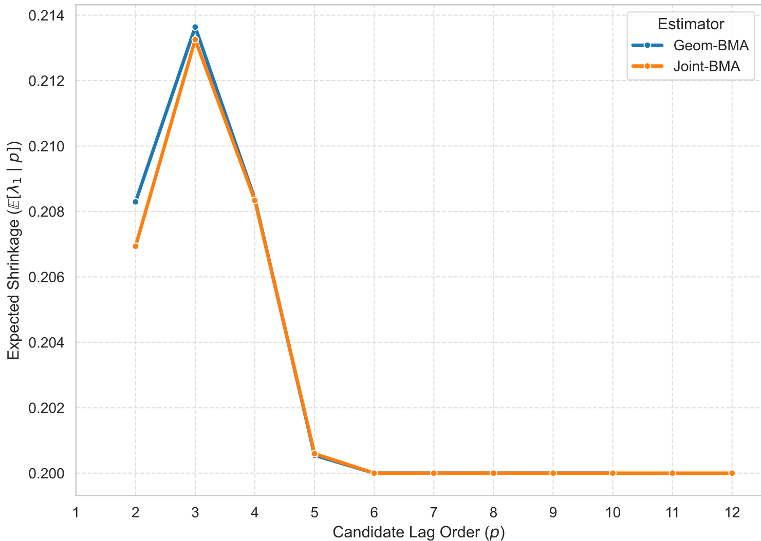
Optimal Shrinkage vs. Lag Order ( T = 600, p_0 = 4 )
