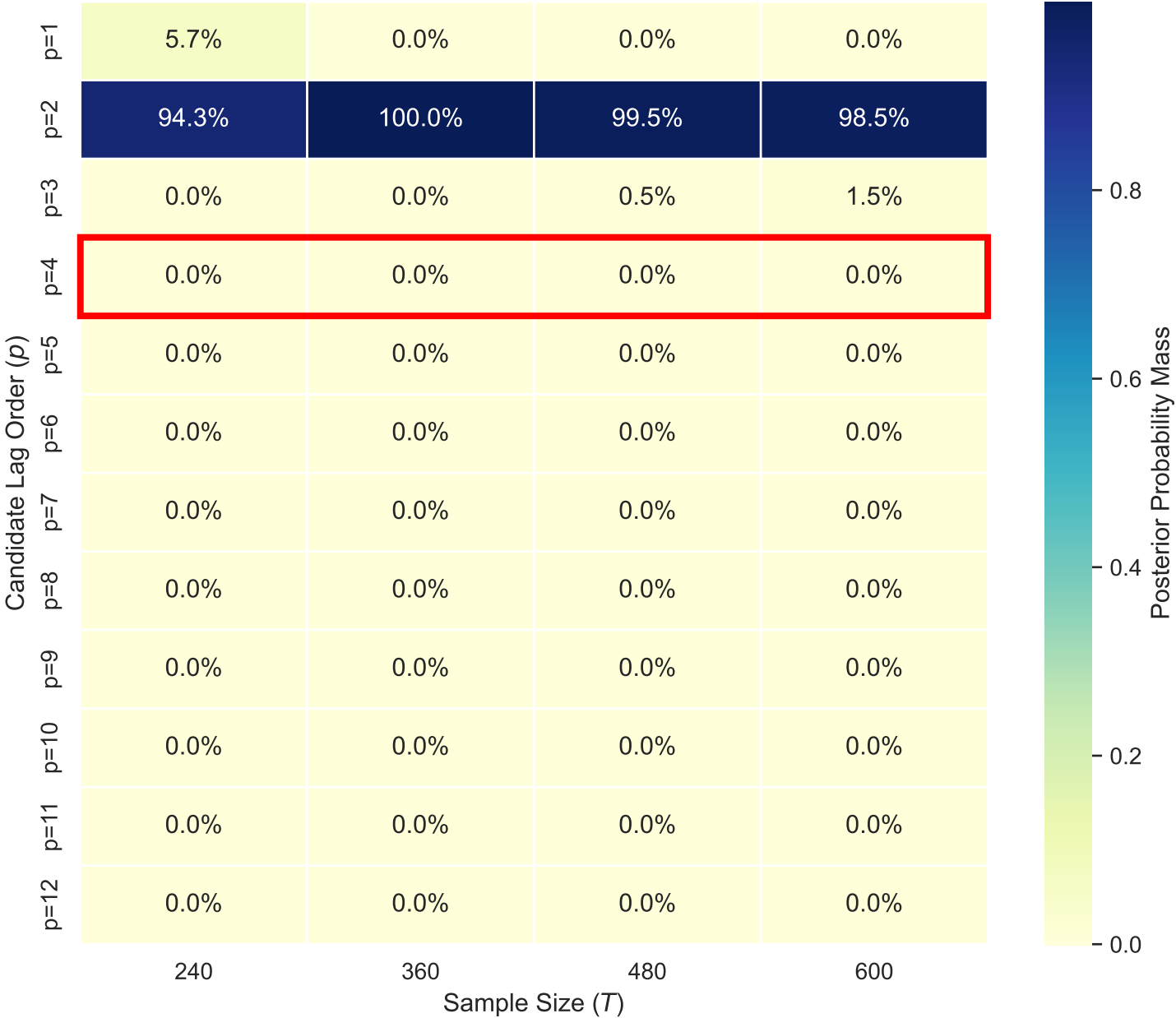
Posterior Weight Evolution: OLS BMA (Geom-BIC-W, \theta = 0.5 ) ( p_0 = 4 )
