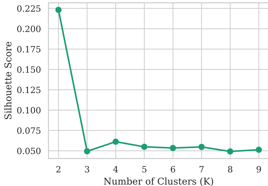
Silhouette Analysis
