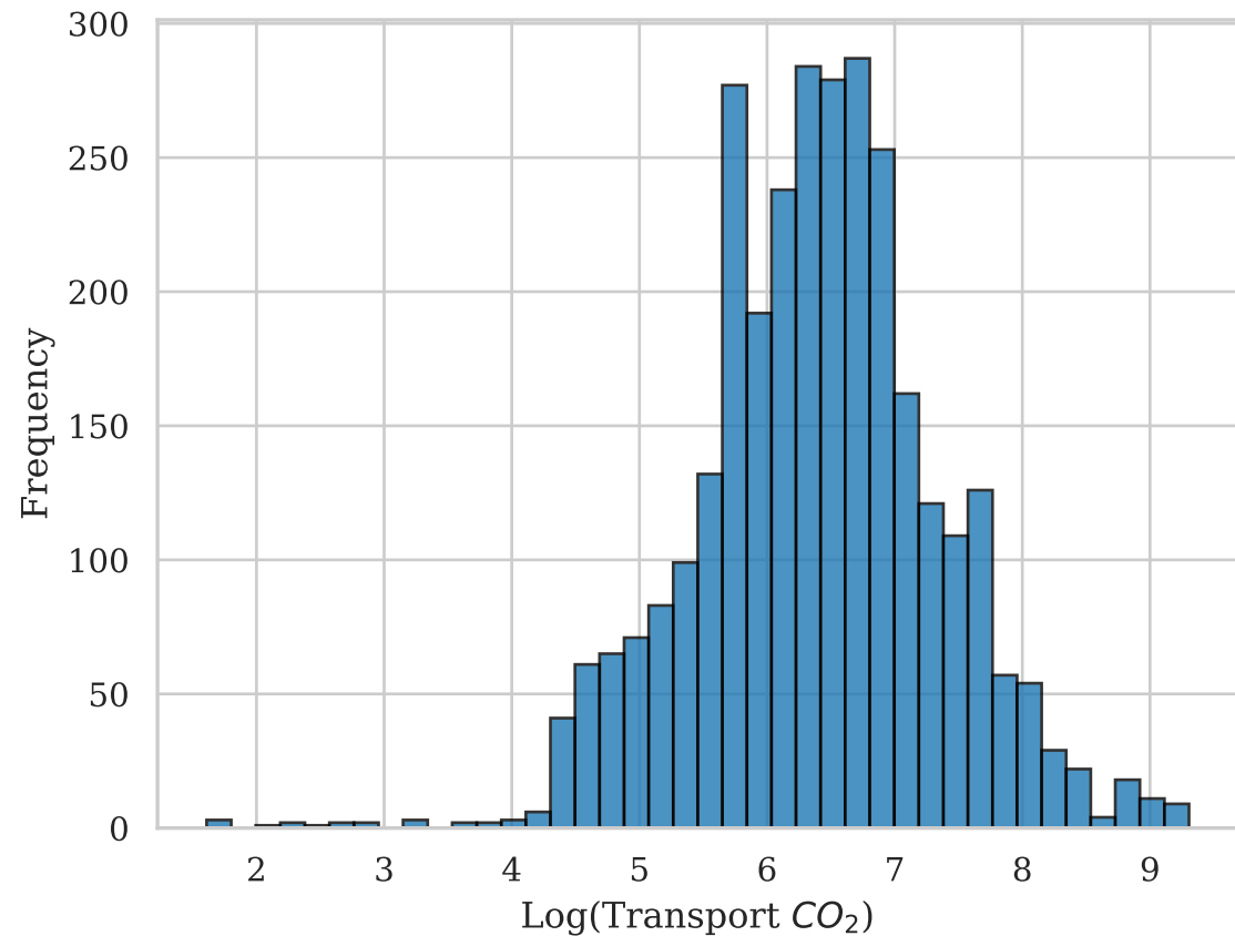
Log-Transformed Distribution
