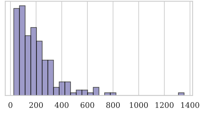
elevation (Skew: 2.54)
