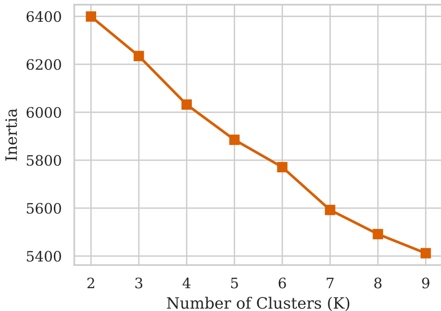
Elbow Method (Inertia)
