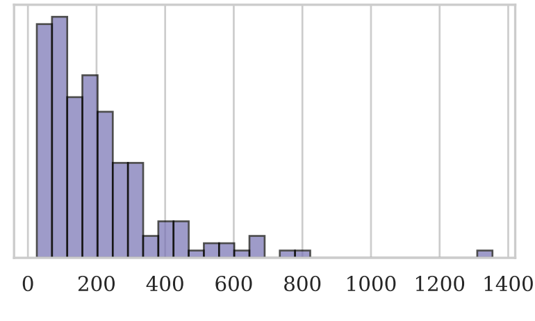
elevation (Skew: 2.54)
