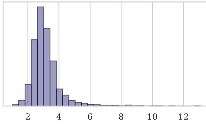
electricity_price (Skew: 1.50)
