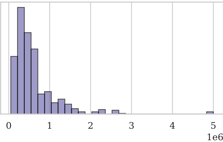
area_km2 (Skew: 1.92)
